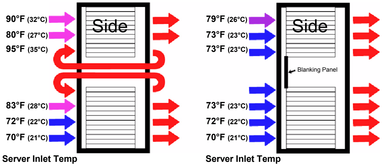
Figure 2 Effect of installation of blanking panels on server air inlet temperature
